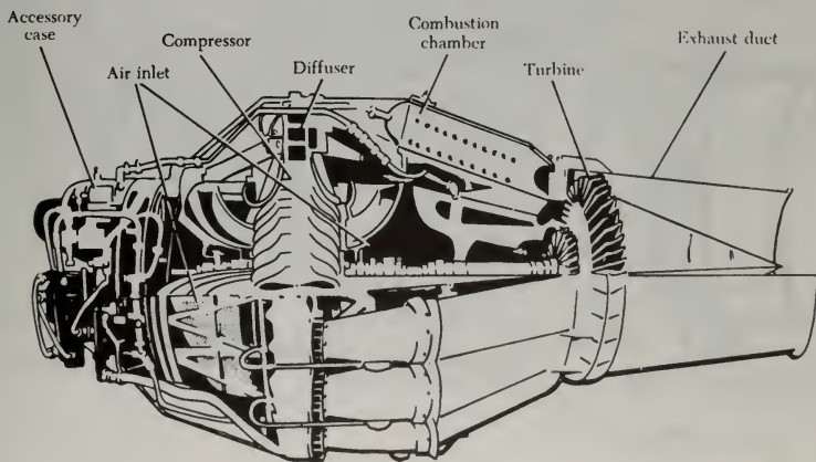
FIGURE 1-33. Centrifugal-flow engine.
